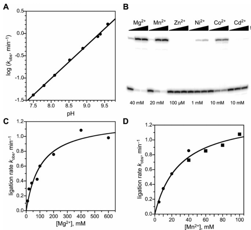
Figure 3. Optimizing incubation conditions for branched RNA formation by 7S11. (A) pH dependence determined at 40 mM Mg 2+ and 37 °C. The slope of the line is 0.74; the fit value of k_{\text{obs}} at pH 9.0 is 0.54 min -1 . (B) Metal ion dependence. The assays were performed at 37 °C and pH 9.0 (Mg 2+ ) or 7.5 (other metals). Time points are 20 s, 5 min, and 20 min for Mg 2+ and Mn 2+ ; 0, 12, and 24 h for the other ions. (C) Determining K_{\text{d,app}} for Mg 2+ at 37 °C. The exact pH of the buffer for this particular experiment was 8.91. (D) Determining K_{\text{d,app}} for Mn 2+ at pH 7.5, 37 °C. The different symbols represent data sets collected in two separate experiments.
