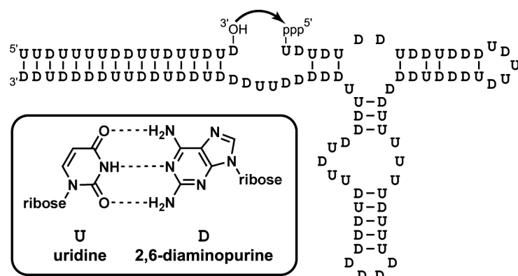
Figure 5 One possible secondary structure of an informationally minimal RNA ligase ribozyme that comprises just two types of nucleotide, uridine (U) and 2,6-diaminopurine (D) (91). The catalyzed reaction is formation of a 3'–5' linkage by reaction of a 3'-hydroxyl group with a 5'-triphosphate. The inset depicts the structures of U and D along with their Watson–Crick base-pairing interaction.
